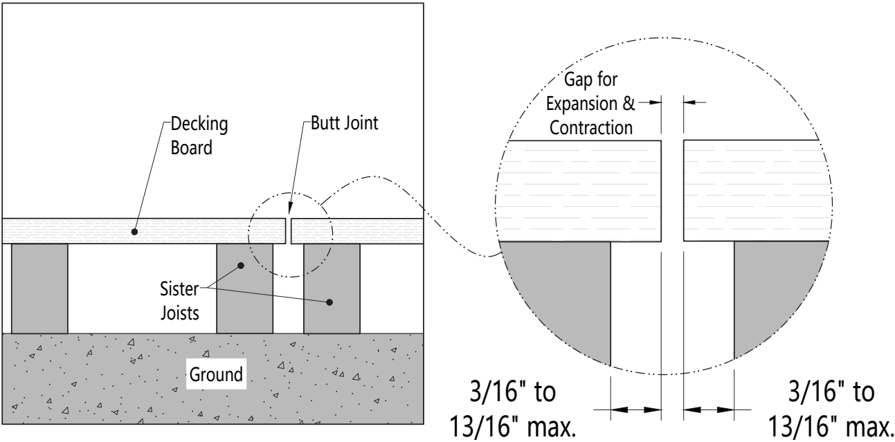
Detail 1-3-1
